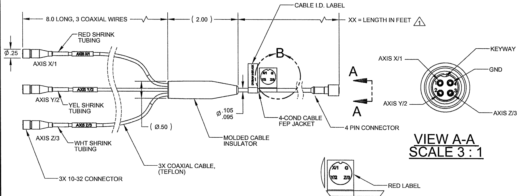
DETAIL B SCALE 1 : 1
